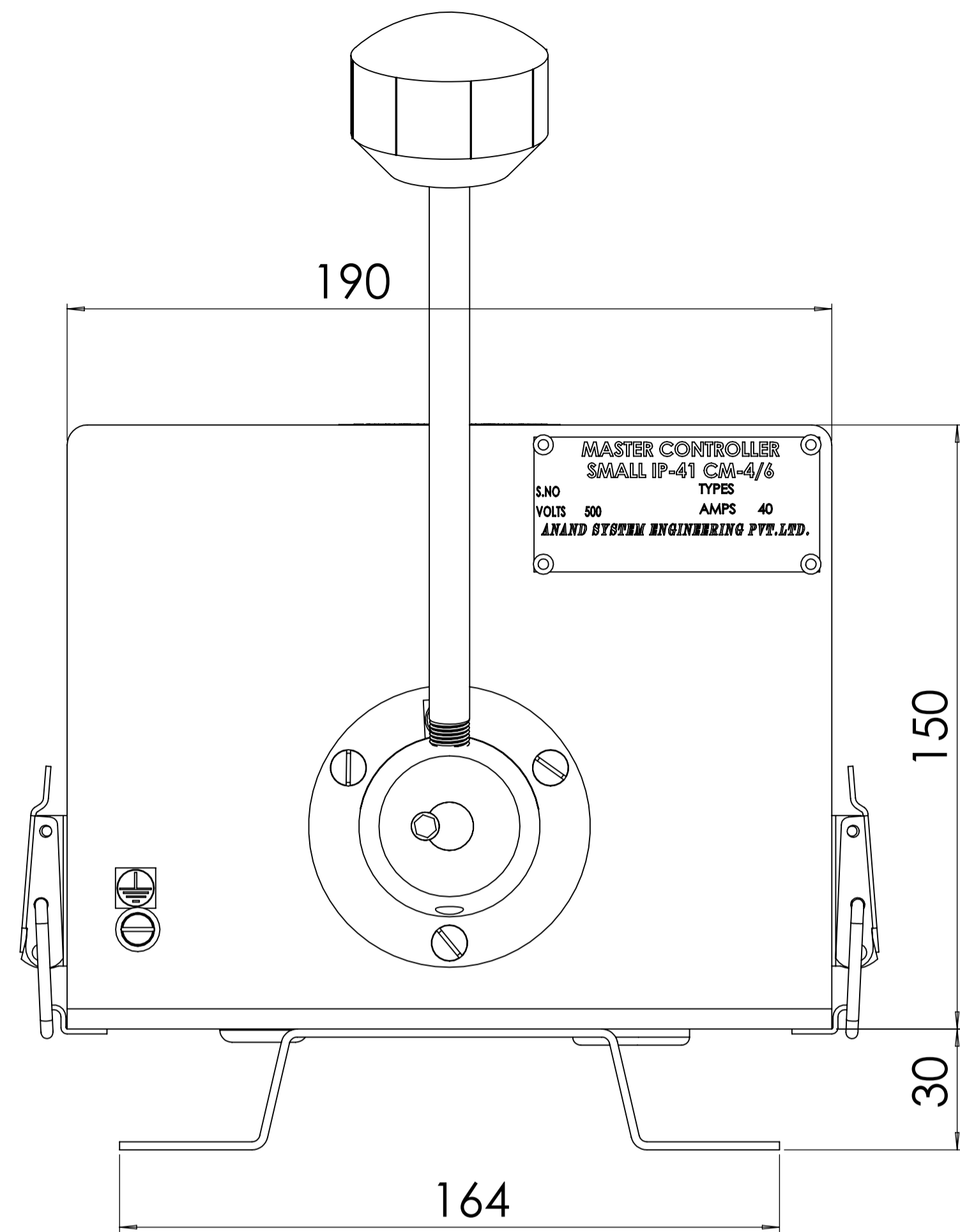
FRONT VIEW
