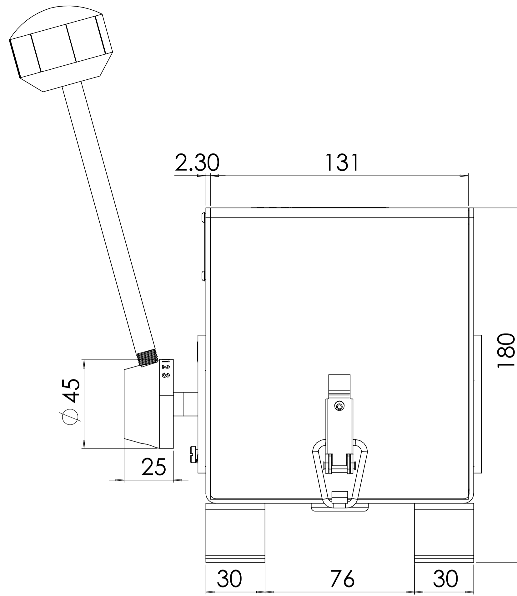
SIDE VIEW
