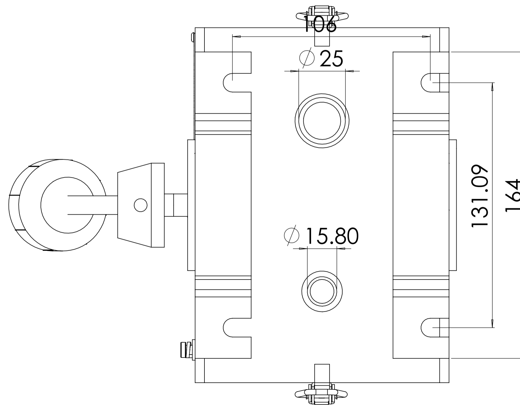
BOTTOM VIEW
