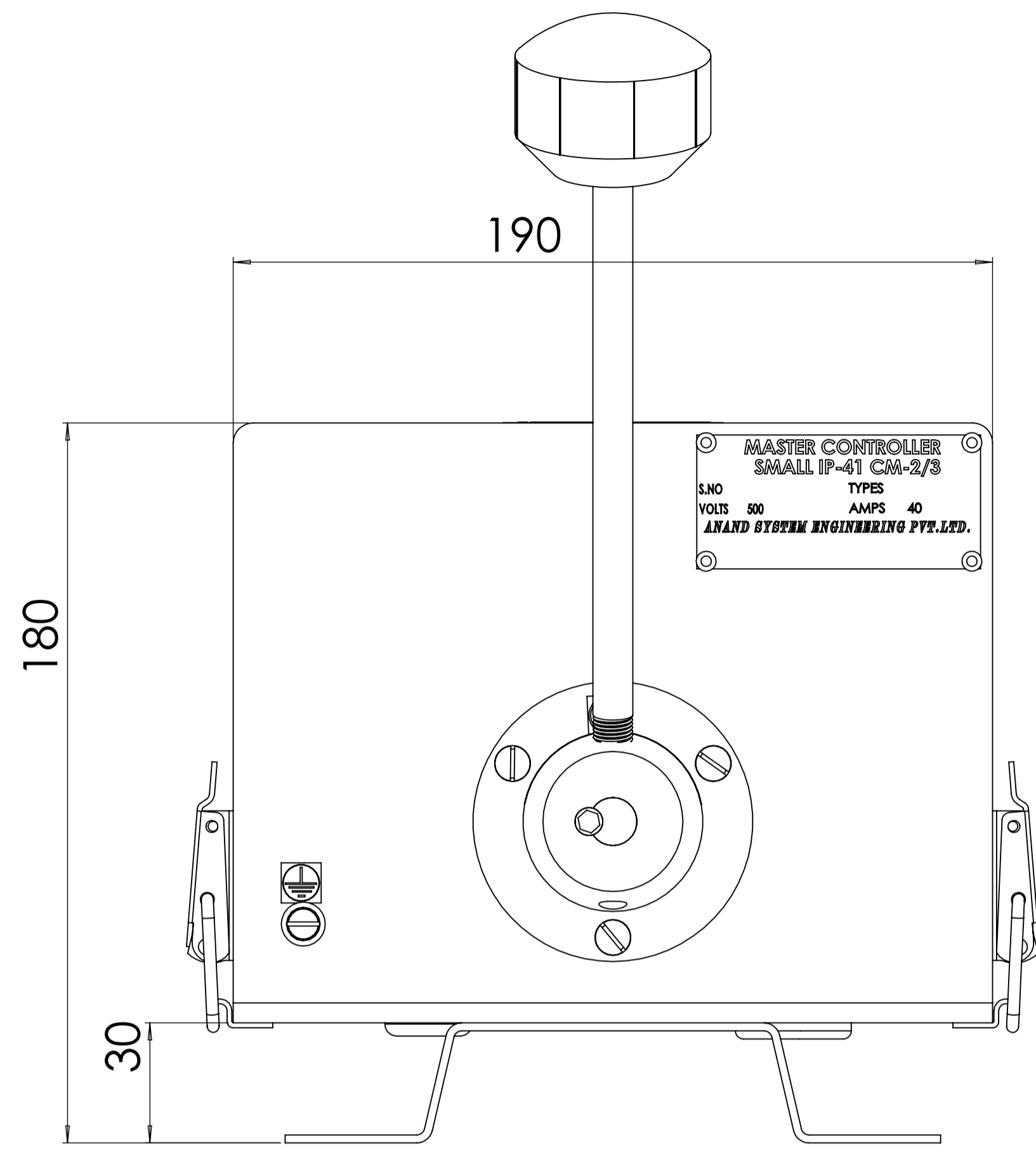
FRONT VIEW
