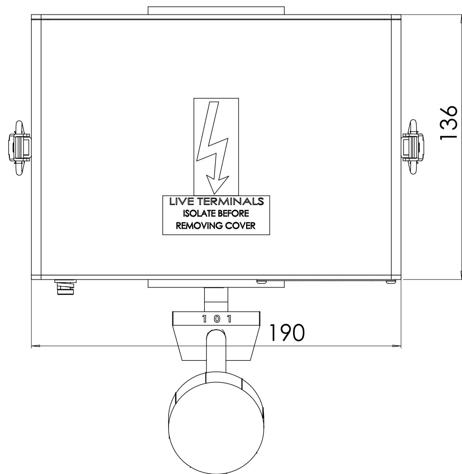
TOP VIEW
