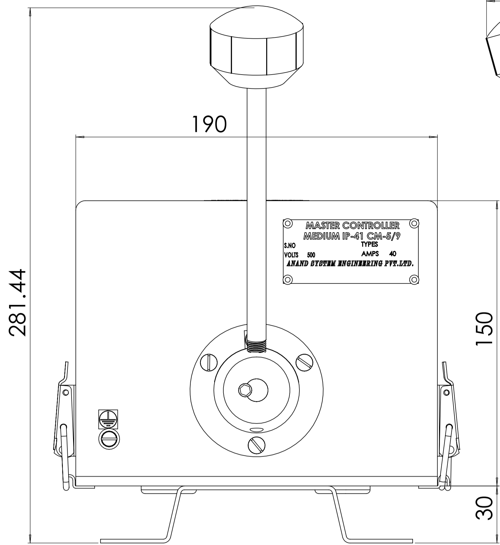
FRONT VIEW
