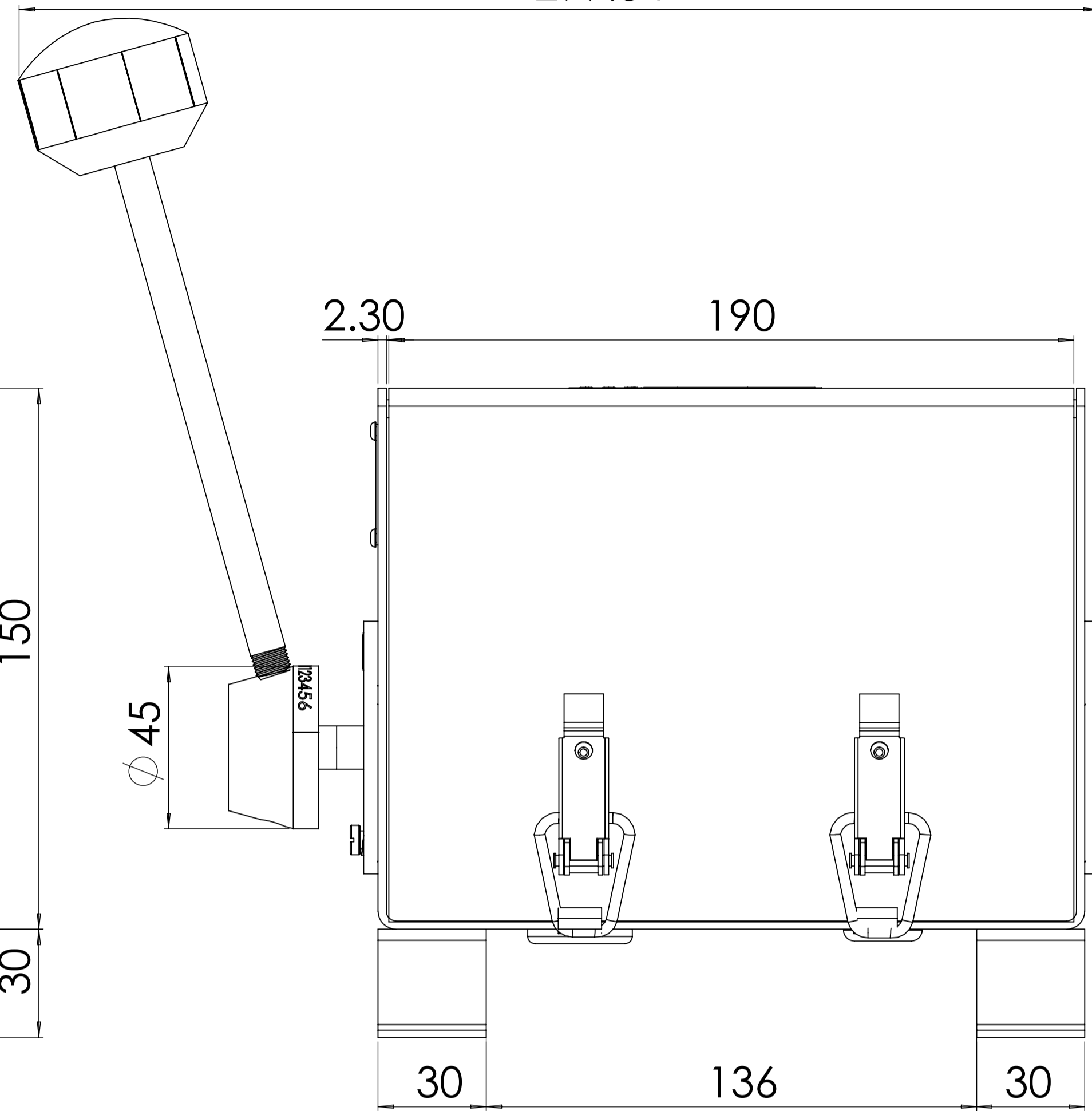
SIDE VIEW 299.54
