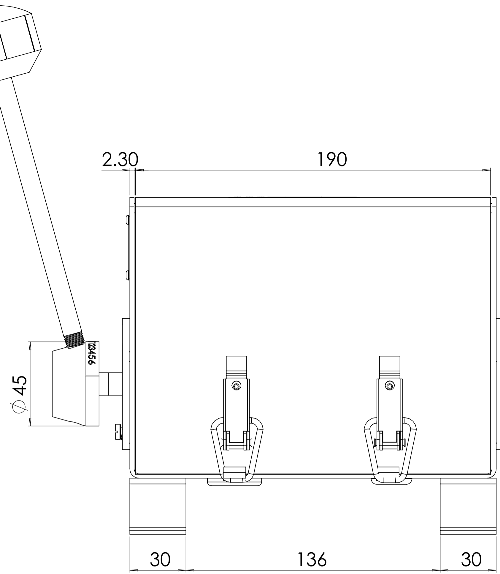
SIDE VIEW
