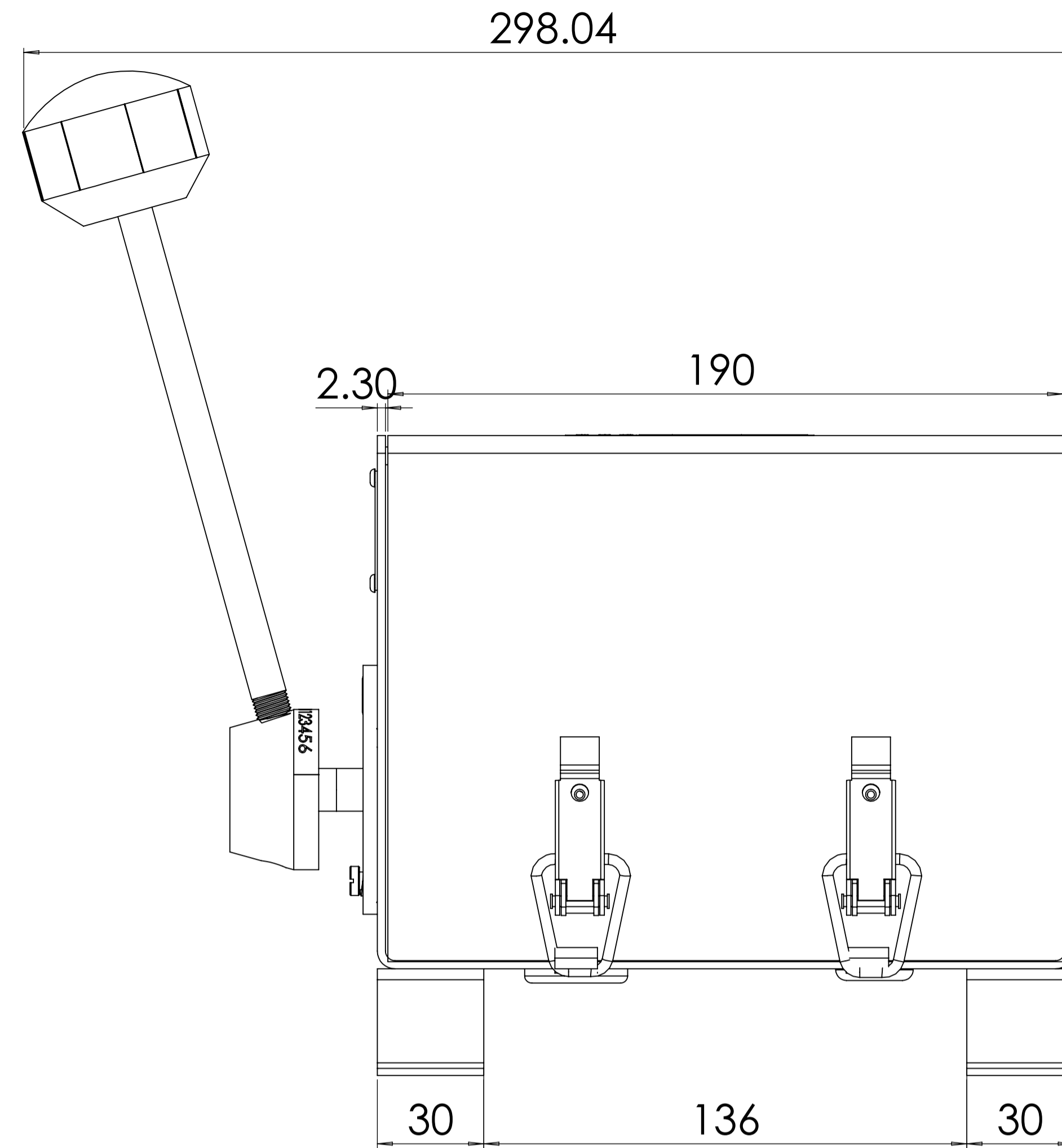
SIDE VIEW
