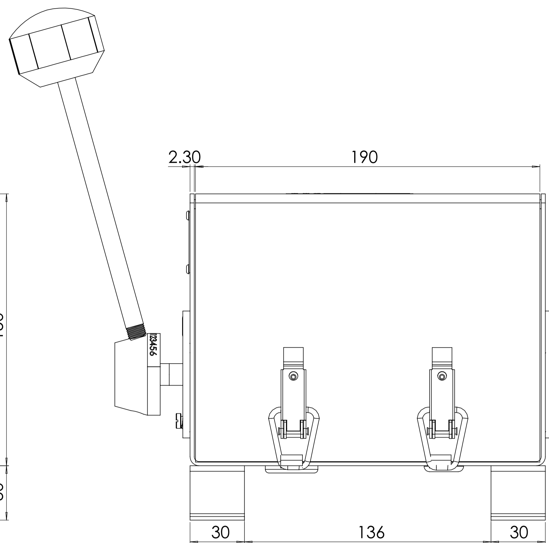
SIDE VIEW
