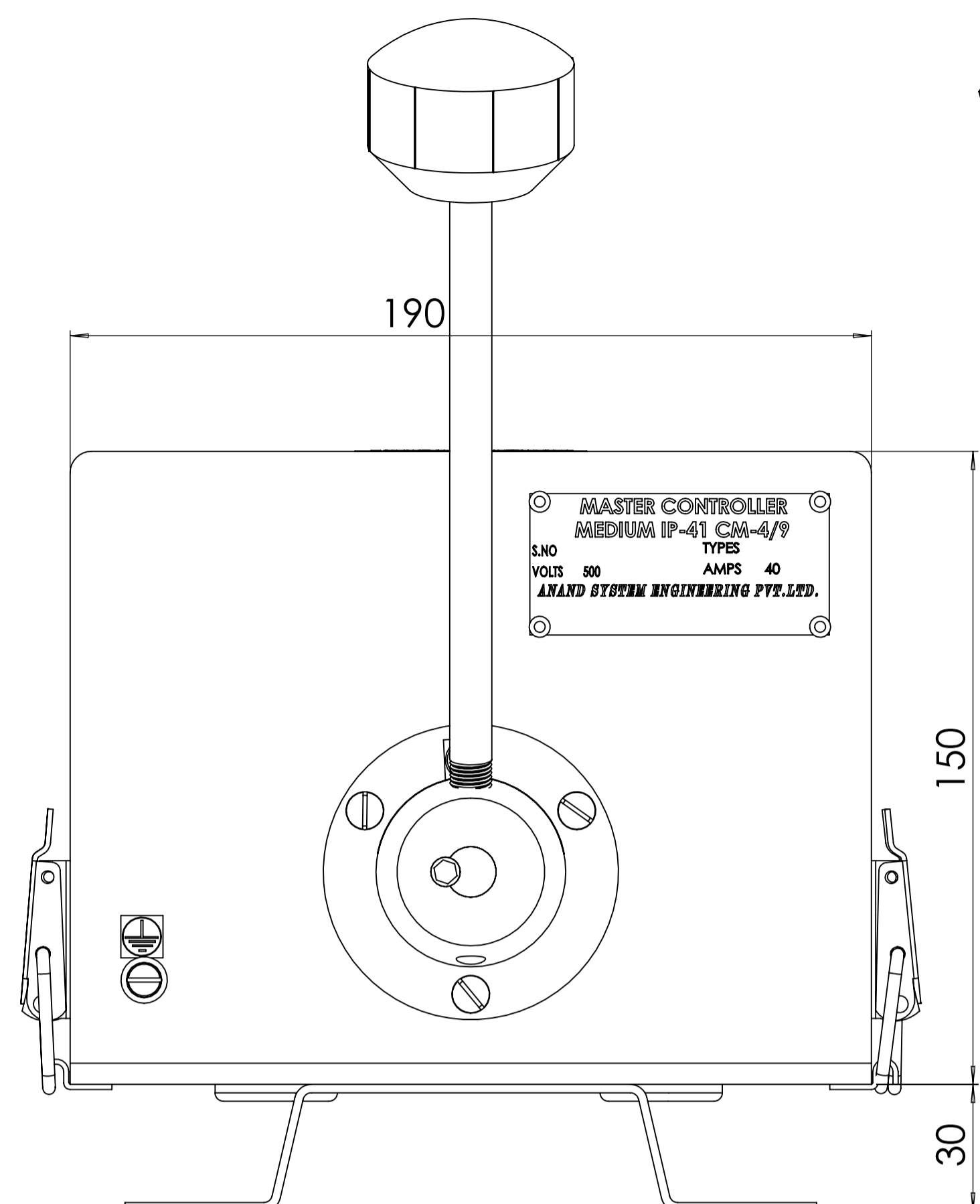
FRONT VIEW
