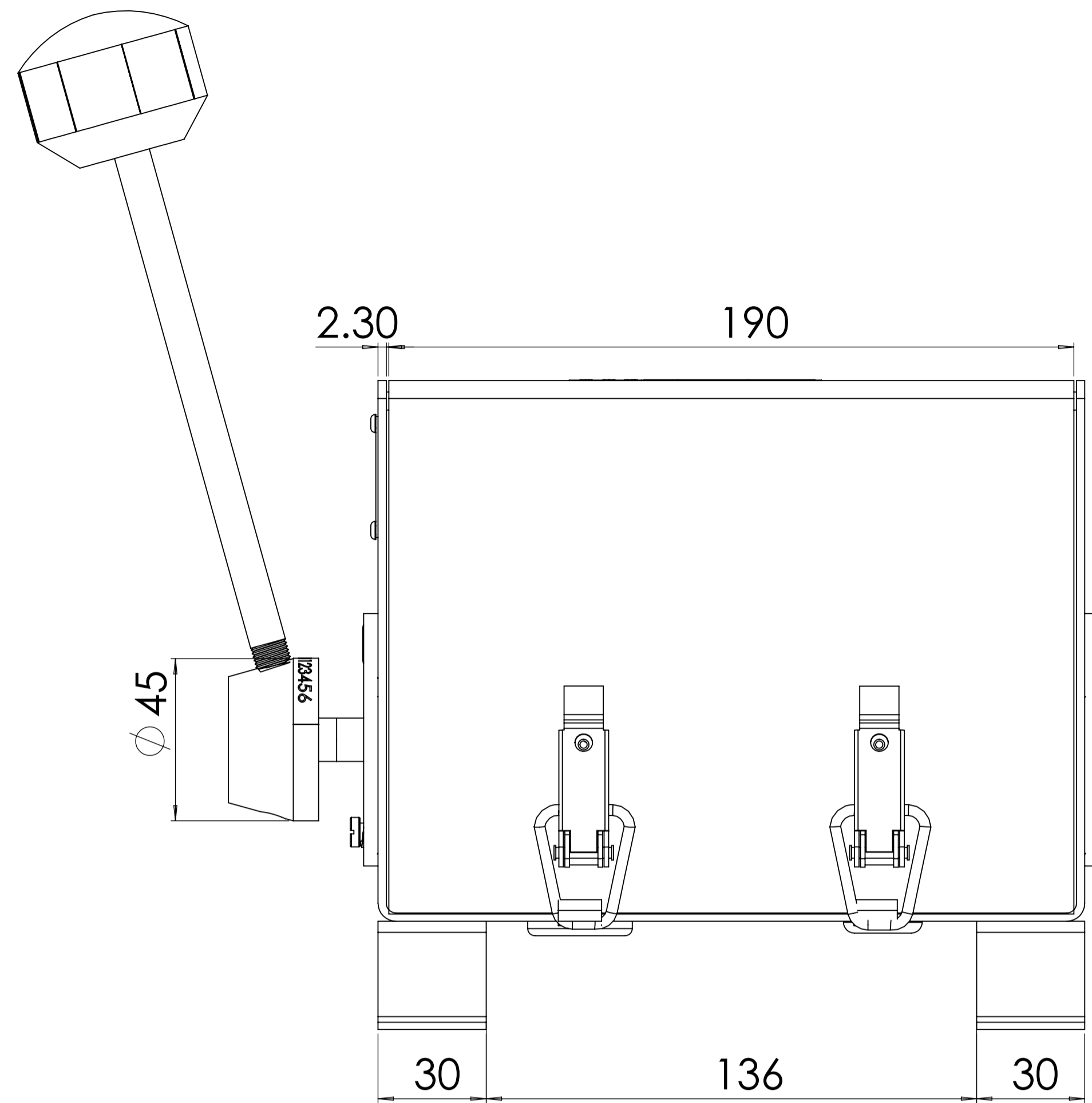
SIDE VIEW
