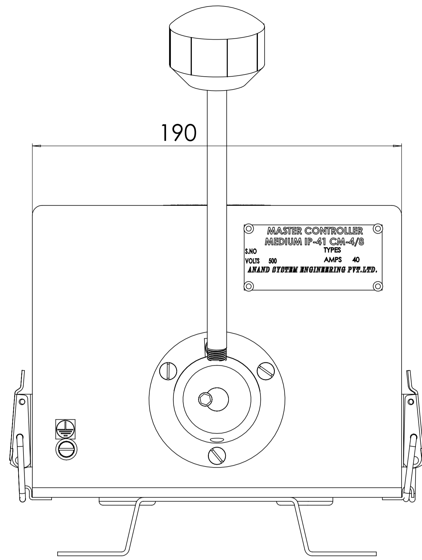
FRONT VIEW
