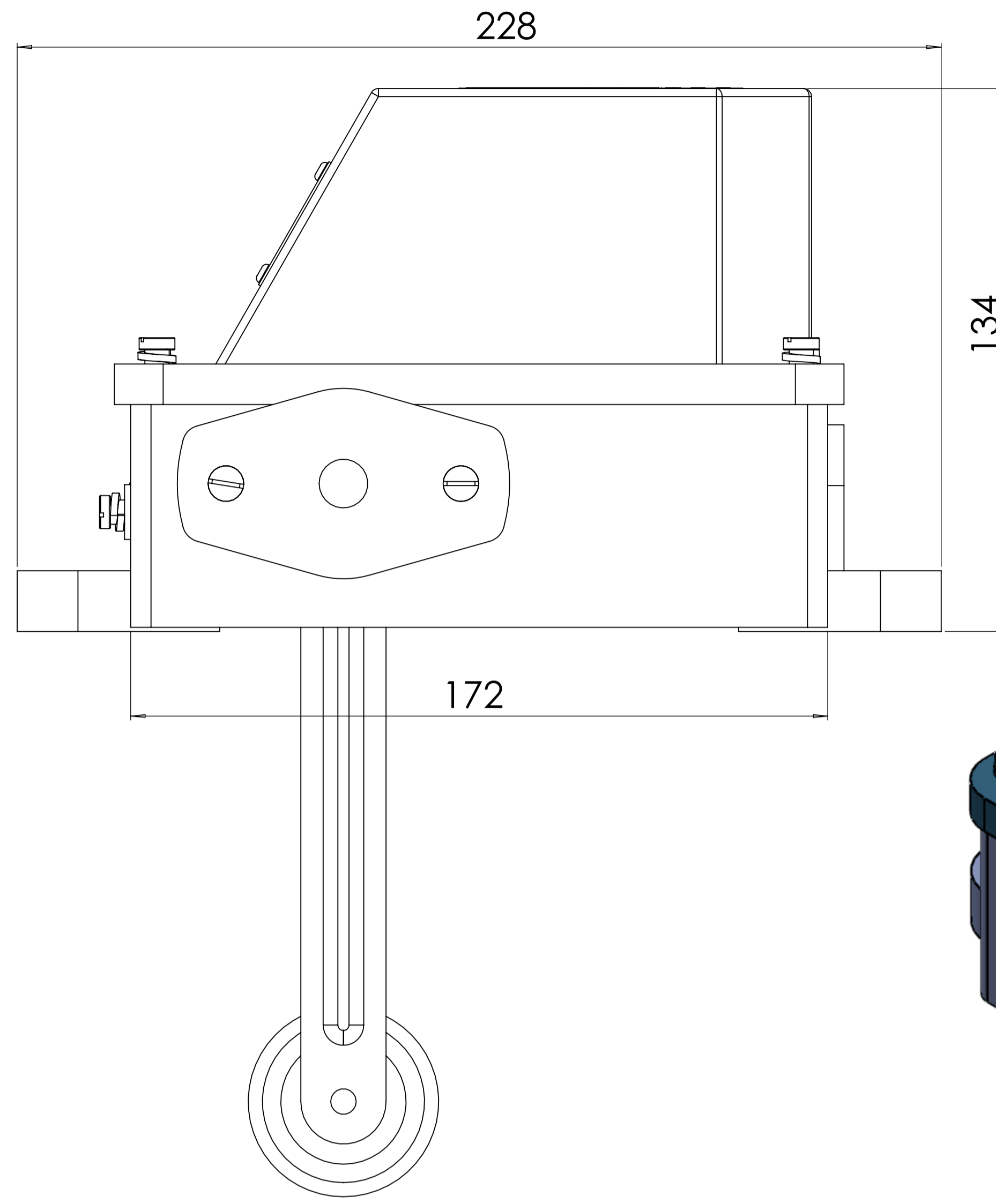
SIDE VIEW
