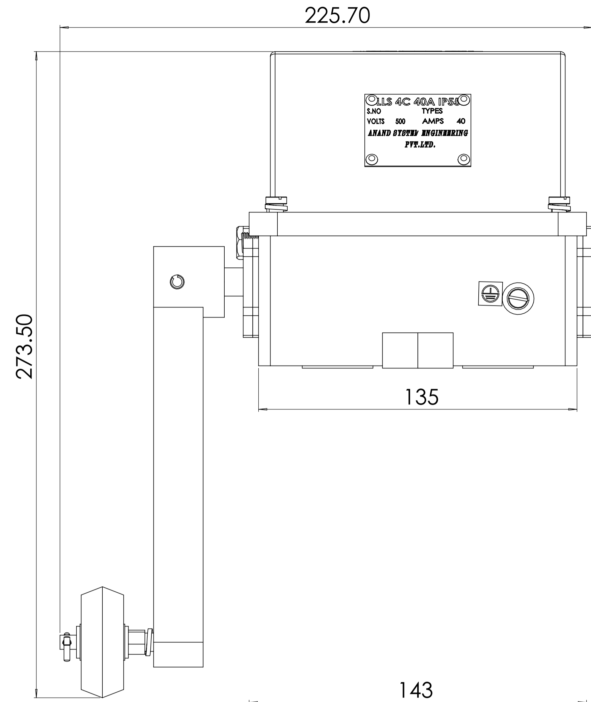
FRONT VIEW
