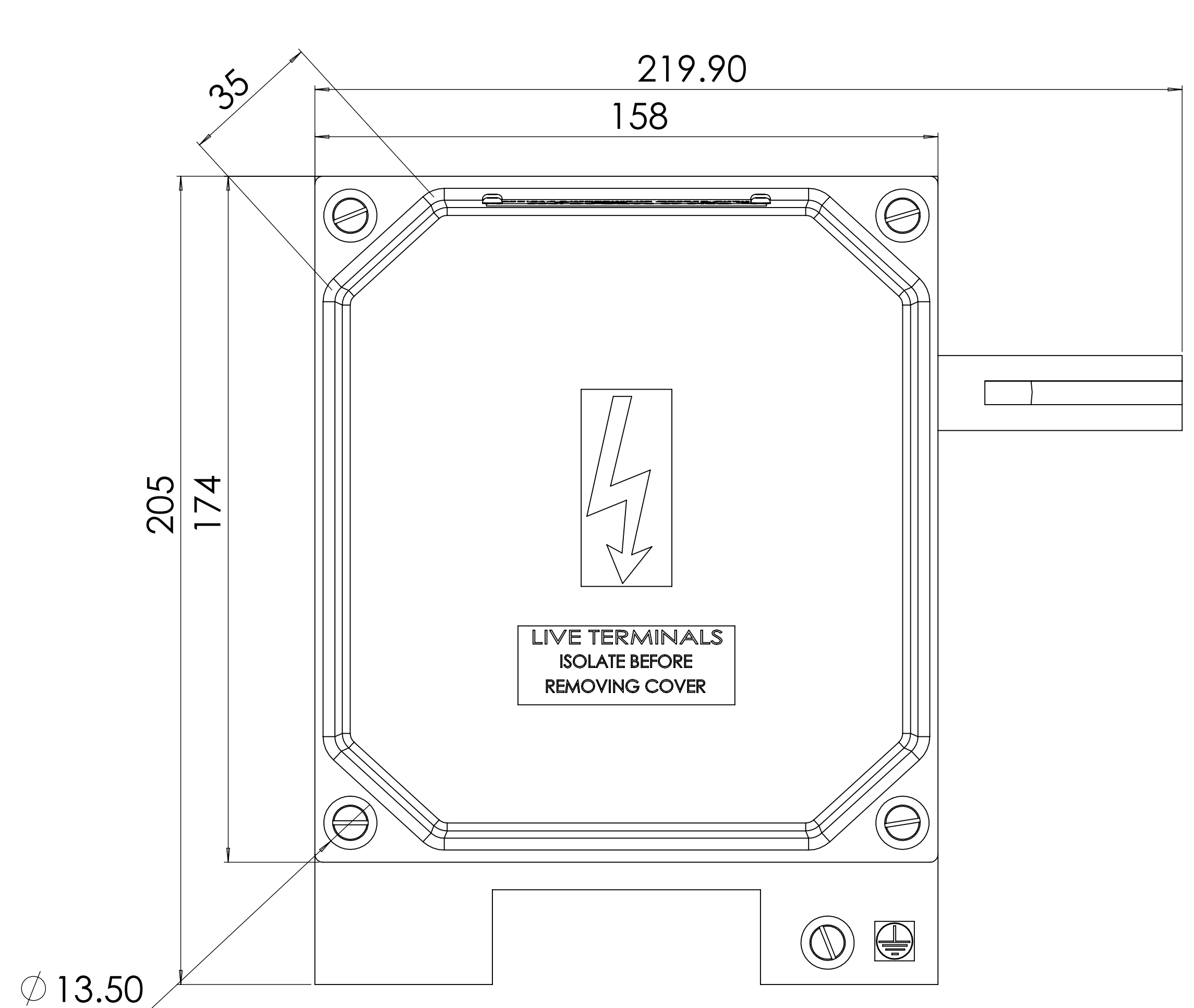
TOP VIEW
