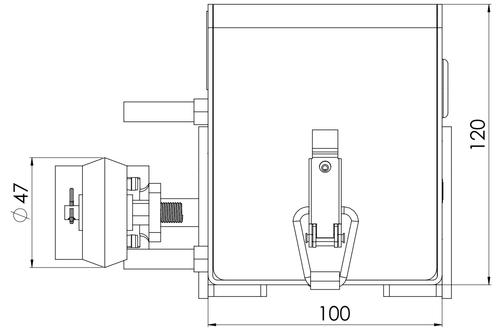
SIDE VIEW
