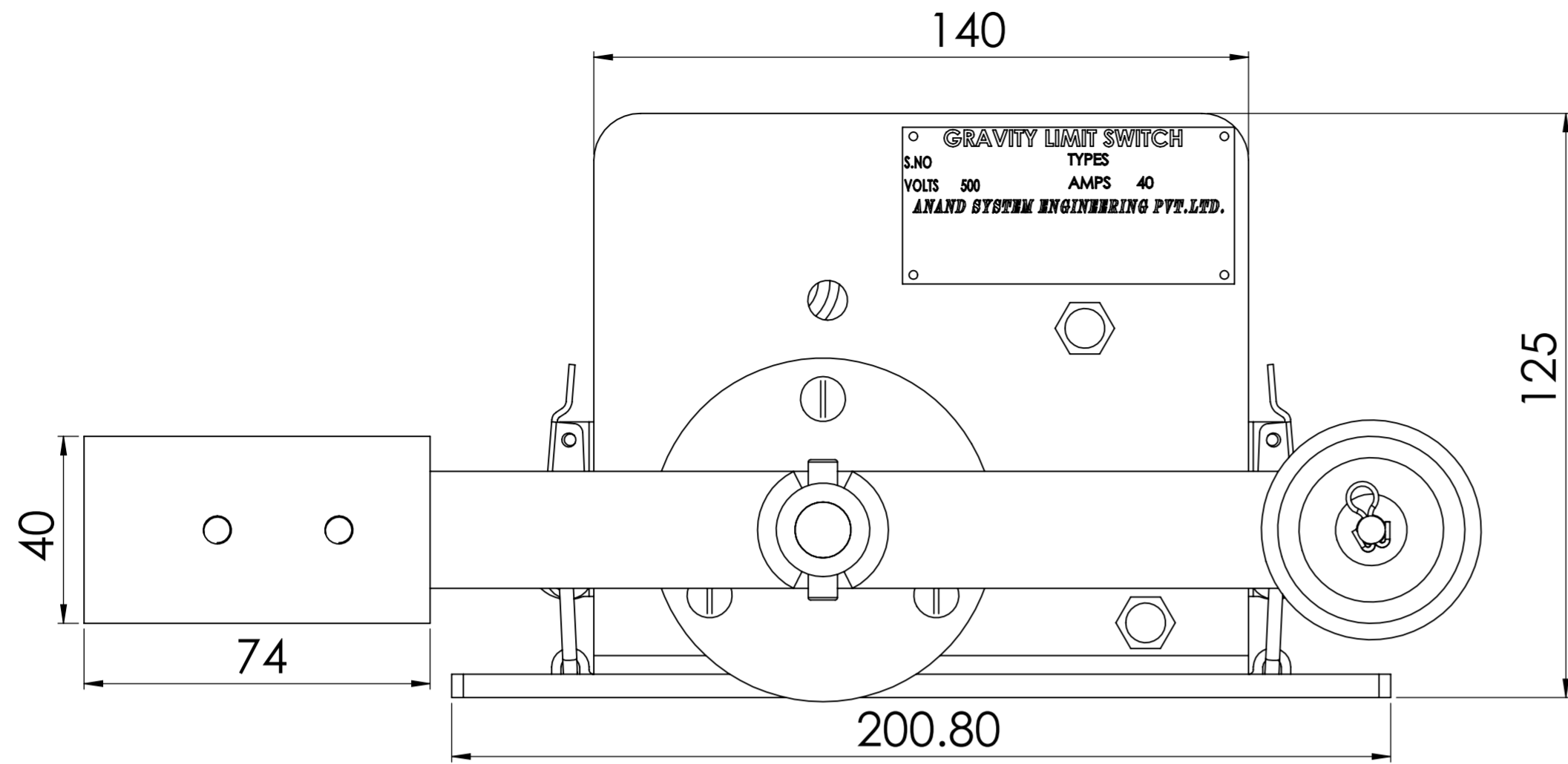
FRONT VIEW
