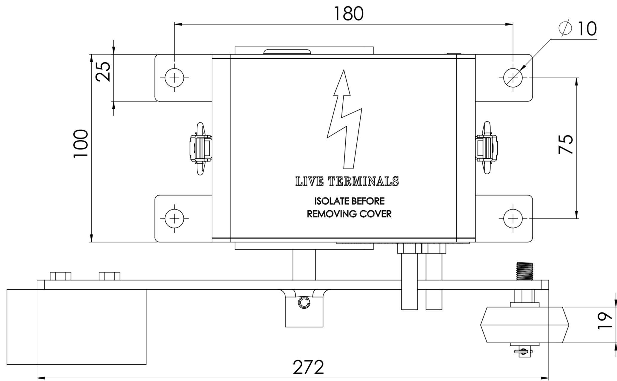
TOP VIEW
