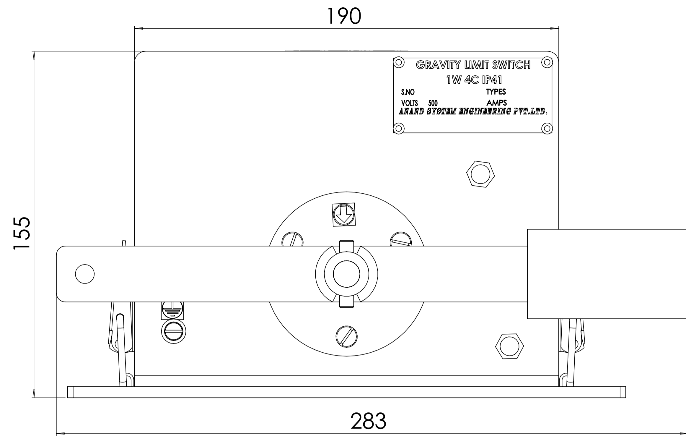
FRONT VIEW
