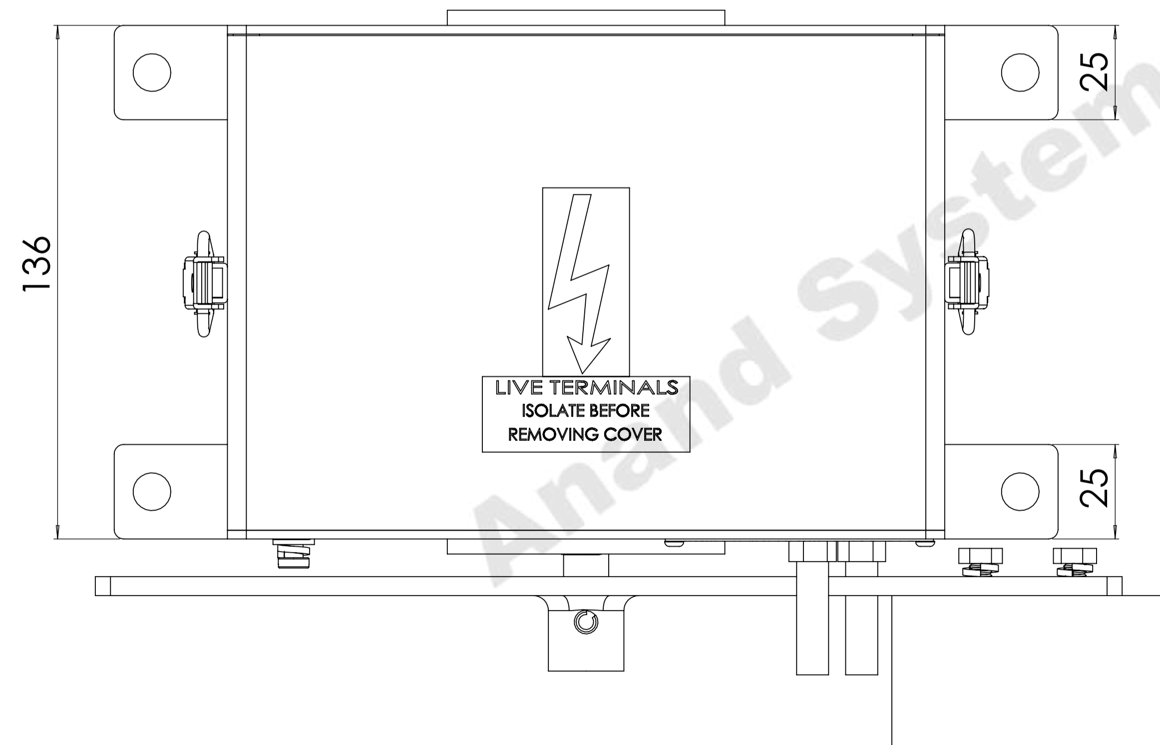
TOP VIEW
