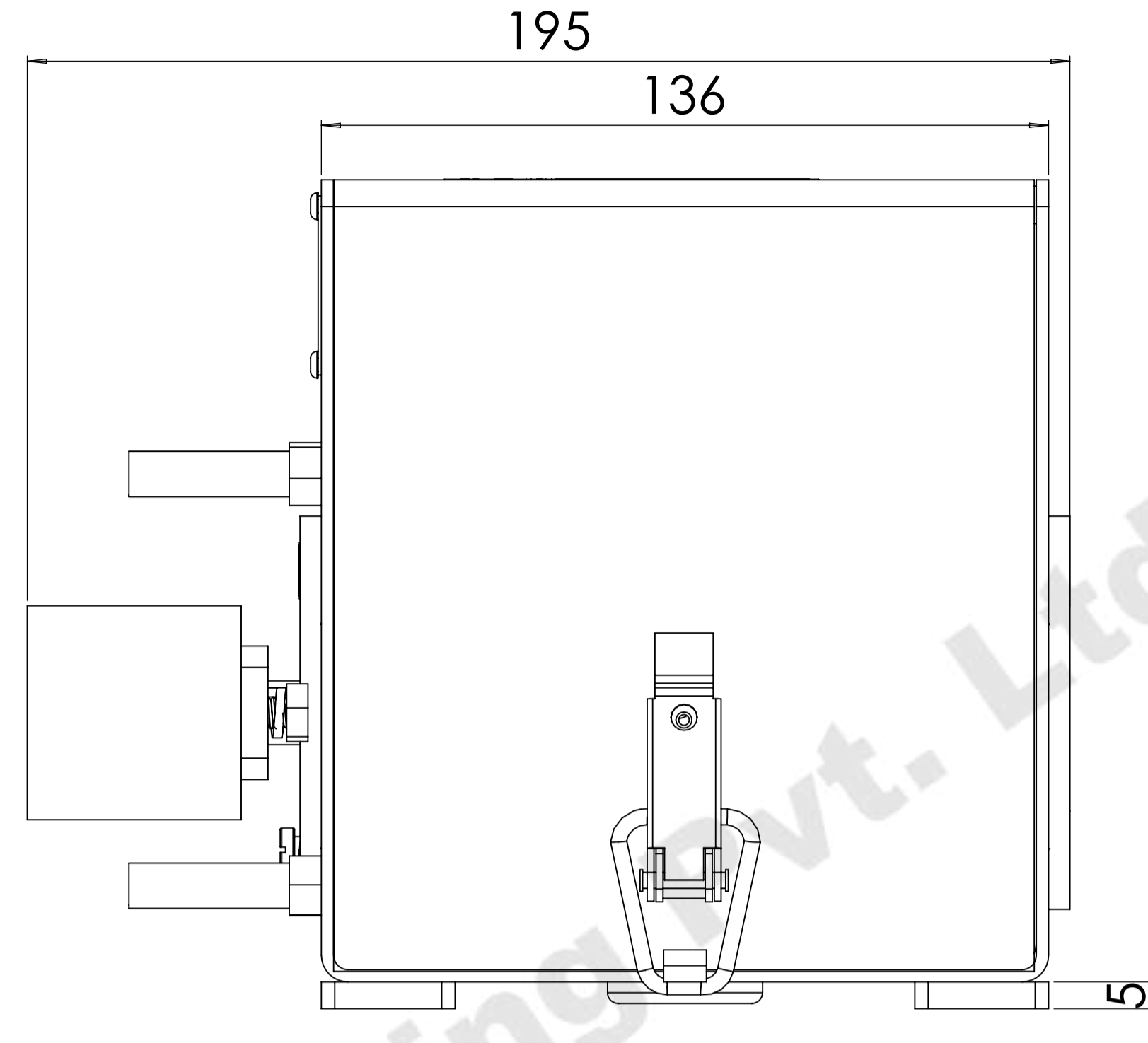
SIDE VIEW
