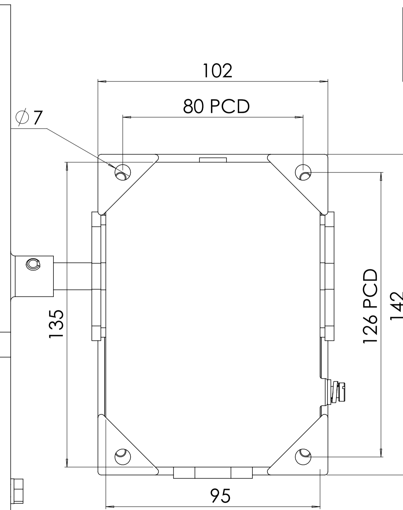
BOTTOM VIEW
