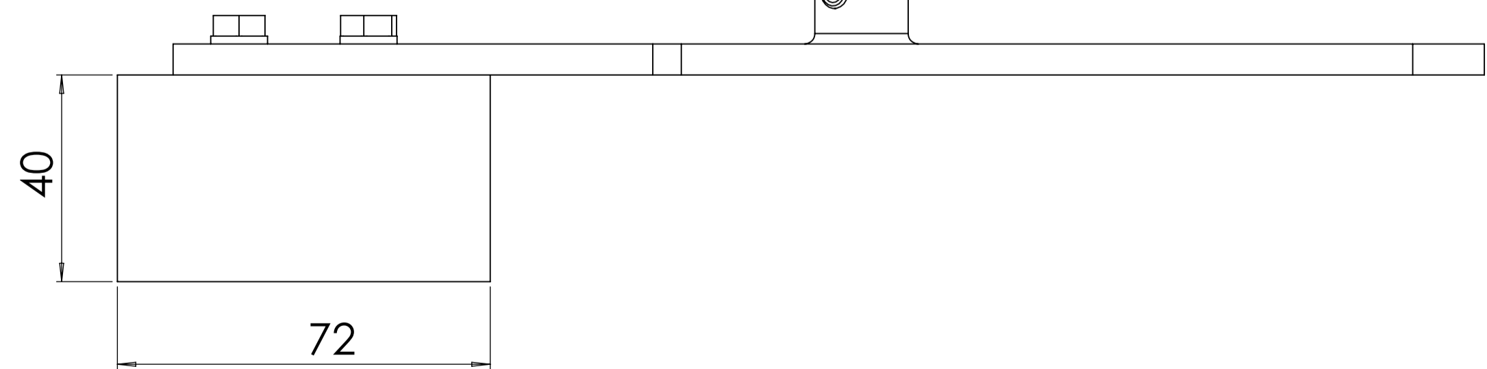
TOP VIEW
